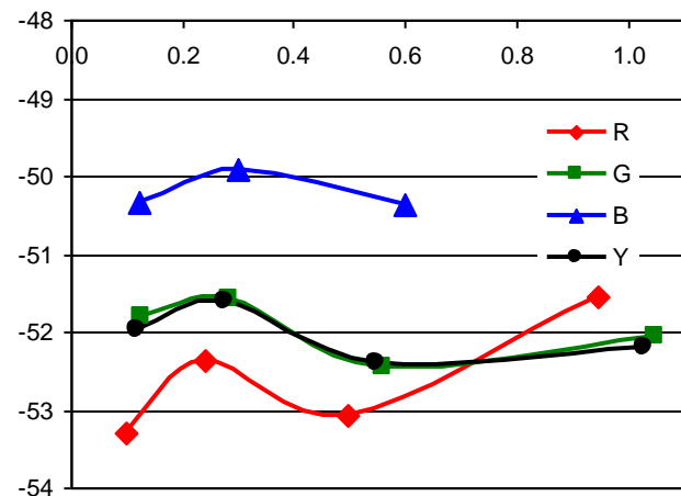
Figure 3 Video noise levels
